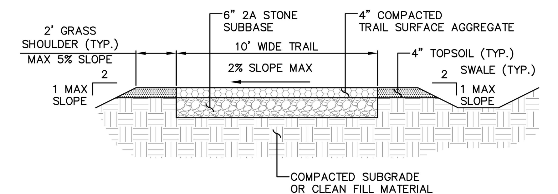
TYPICAL TRAIL CROSS SECTION NOT TO SCALE
